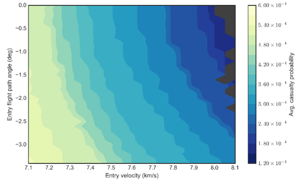
Figure 3. Casualty risk as function of entry velocity and flight path angle for a 120 inclination orbit.
