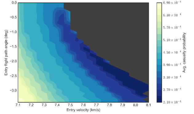
Figure 2. Casualty risk as function of entry velocity and flight path angle for a 30 inclination orbit.
