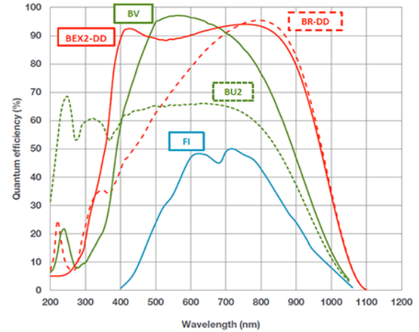
Figure 3: Quantum efficiency of the various models of the IKON L936 ANDOR cameras (courtesy ANDOR).
