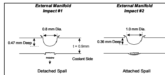
Figure 3. Impacts on STS-86 radiator interconnect lines.
