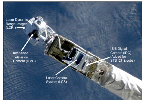
Figure 10. OBSS sensor suite
