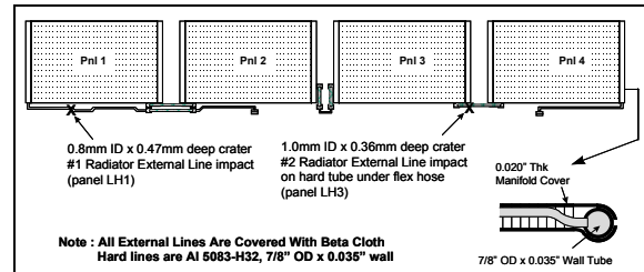
Figure 2. Impacts on STS-86 LH radiator interconnect lines.
