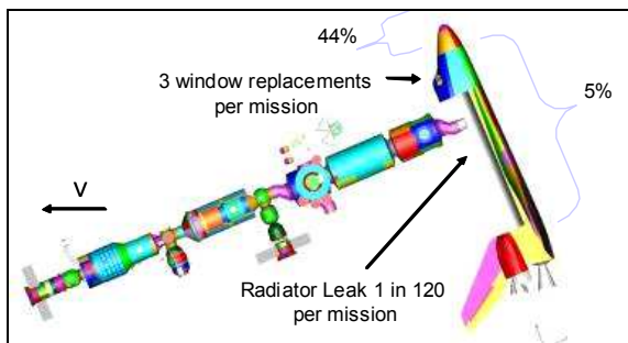
Figure 8. ISS -XVV mated attitude, reduced MMOD impact risk to lower TPS, residual risk concentrated on nose cap
