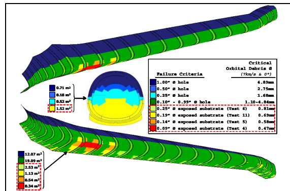
Figure 6. Post-STS-107 RCC failure criteria map.
