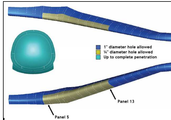
Figure 5. Pre-STS-107 RCC failure criteria map.
