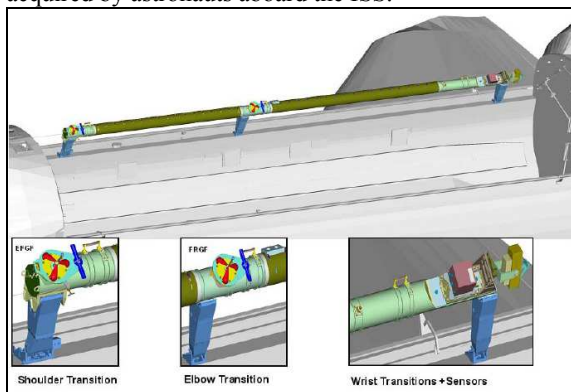
Figure 9. Orbiter Boom Sensor System.
