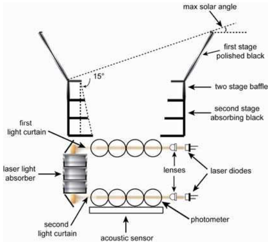
Figure 6. An illustration of the basic configuration of the second IMMUSE component, SEDS.
