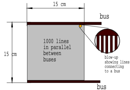
Figure 1. An illustration of the RGS system design.
