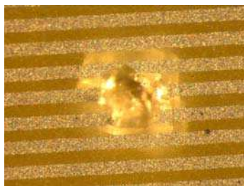
Figure 2. Damage caused by a 100 μm glass particle at 5 km/s normal impact on a test RGS unit.
