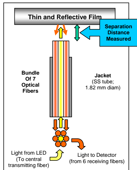
Figure 3. An illustration of the detection principle of the fiber optic displacement sensor.
