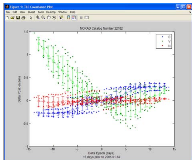
Figure 1. VNC Error vs. Delta Epoch Time
