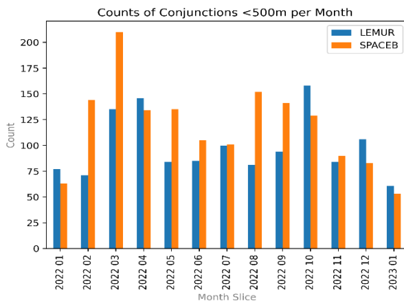
Figure 2. Example Monthly Statistics of Conjunctions <500m for selected fleets/operators: LEMUR (Spire) and SpaceBEE (Swarm Technologies)
