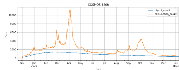
Figure 1. Example Object vs. Conjunction Count <5km (Cosmos-1408)
