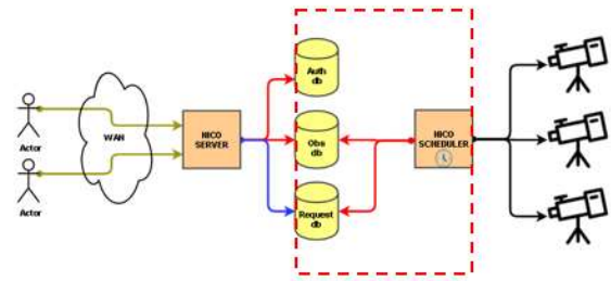
Figure 14. NICO Back-End layer flowchart.
